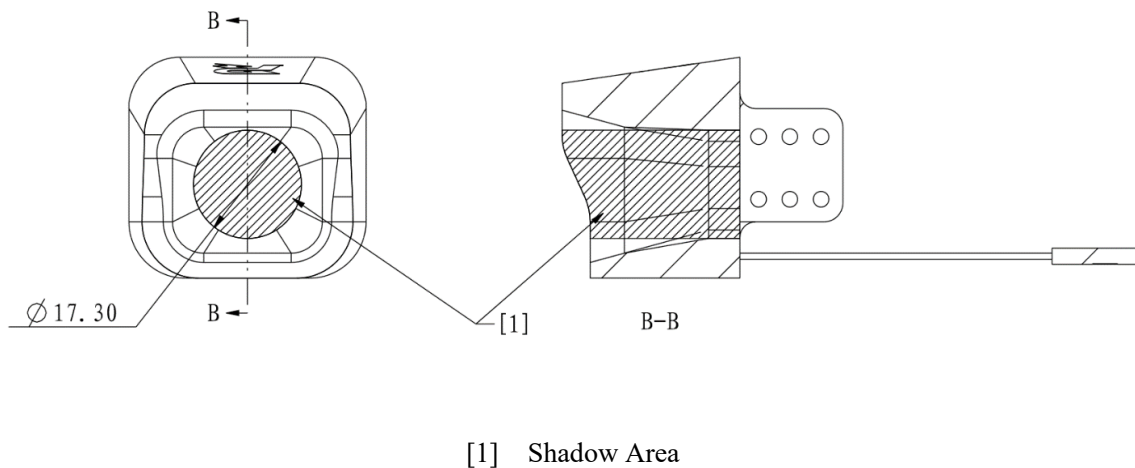
Figure 2-5 Dart Trigger Device internal cavity is blocked
