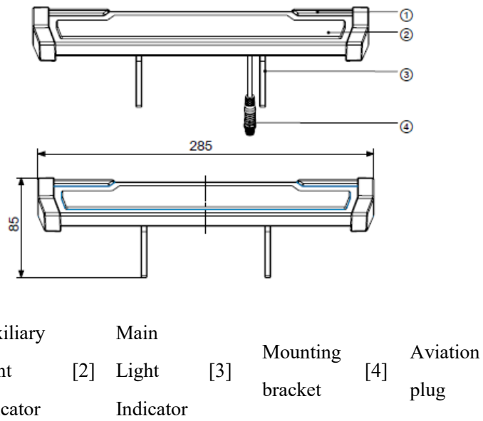
Figure 3-9 Light Indicator Module
