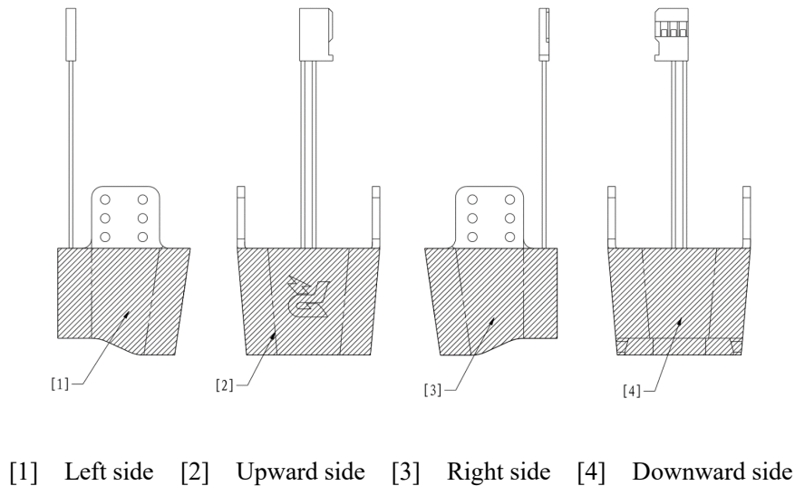
Figure 2-4 Dart Trigger Device is blocked
