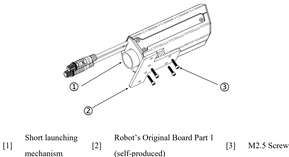
Figure 3-34 Mounting 17mm short launching mechanism
