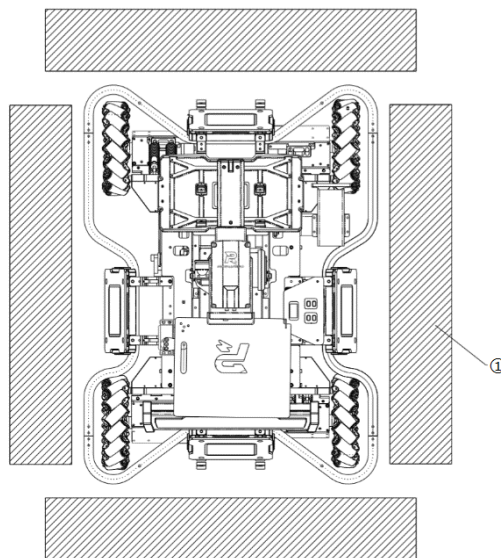
[1] Wall
